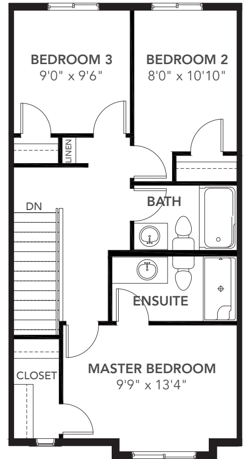
SECOND FLOOR 600 SQ FT
