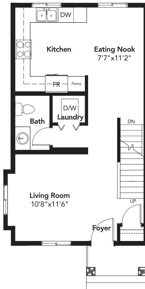
MAIN FLOOR 586 SQ FT
