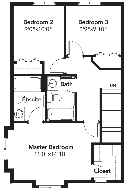
SECOND FLOOR 620 SQ FT
